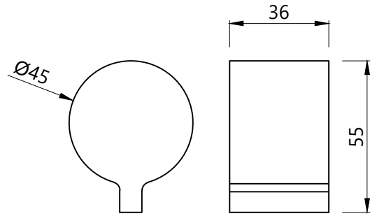
DIVERTER HANDLE
