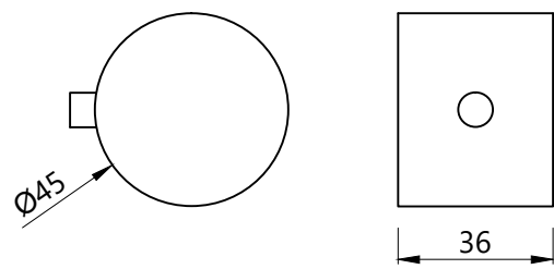
THERMOSTATE HANDLE
